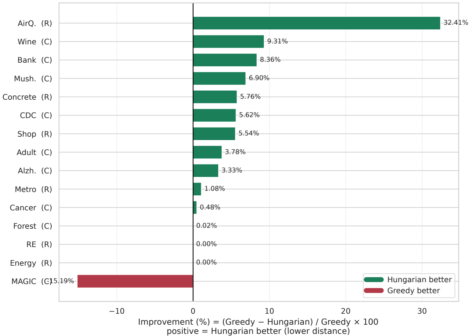
Figure 3. Hungarian improvement over Greedy by dataset
